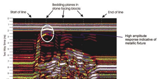
Figure 1(d). GPR survey of Middlesbrough Town Hall Clock Tower. Example radargrams
