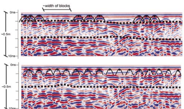
Radargrams collected over two supporting columns. Differences in block geometry and reinforcement prove that these columns were constructed in different ways, and confirmed previous suspicions that they had been constructed at different times
